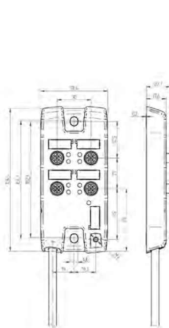
ASB-R 4/ASB-R 4... LED
