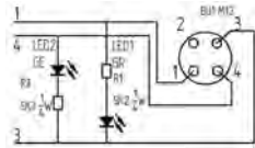
WRST-WRKT/LED A (pnp-Schließer)
