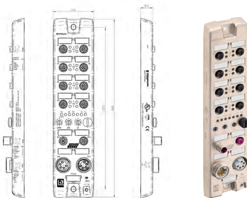
0970 PSL 812-PB-DP 16DO-M12-R
