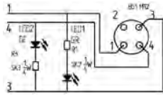
WRKWT/LED A 4-3-250/...M (3-polig)
