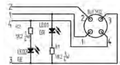
WRST-WRKT/LED F (pnp-Schließer)
