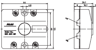
0911 ANC 401 *a = LINE 1 *b = LINE 2
