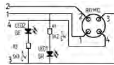
WRKWT/LED F 4-521/...M (4-polig)
