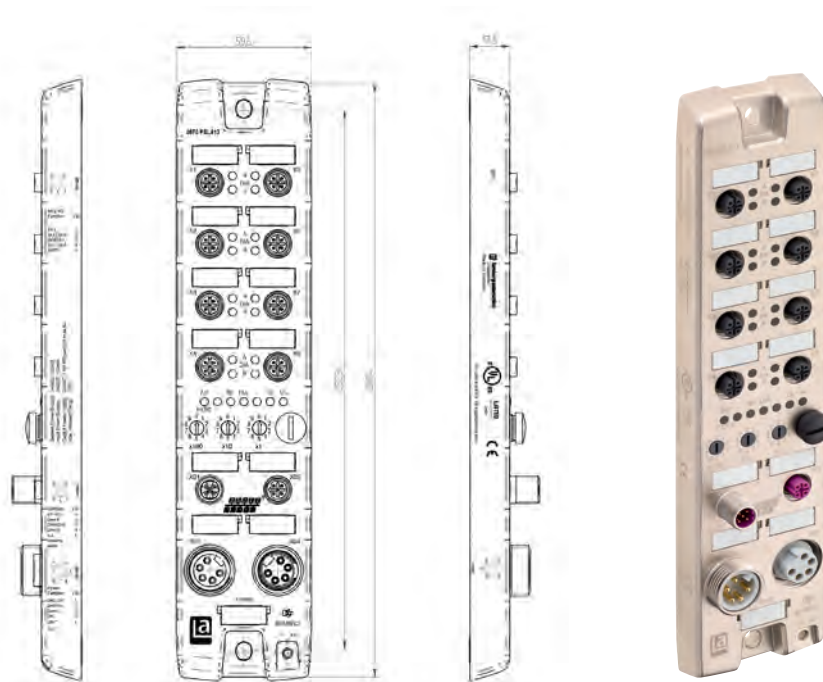
0970 PSL 813-PB-DP 8DI8DO-M12-R
