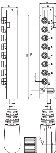
RSWU 12-SB 8/LED 3-333
